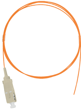
NMF-PT1M2C0-SCU-XXX-001-2 MM 50/125 OM2, SC/UPC-Empty, LSZH, D=0.9mm, 1m
