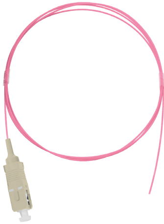
NMF-PT1M4C0-SCU-XXX-001-2 MM 50/125 OM4, SC/UPC-Empty, LSZH, D=0.9mm, 1m
